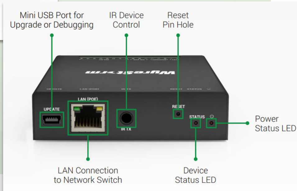
Rear Panel
