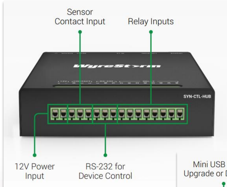
Front Panel
